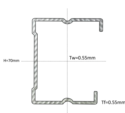
DF 70mm Horizontal Connector
