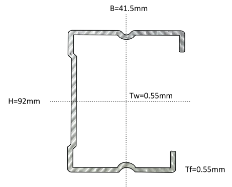
DF 92mm Horizontal Connector
