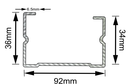
DF-GI-Stud - 92mm Premium
