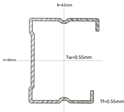
DF 48mm Horizontal Connector
